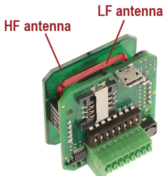
PCB contained in TWN4 Palon Compact LEGIC Wall Light
